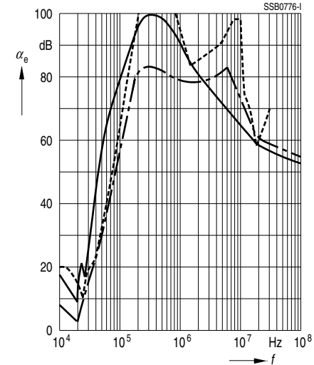
B84142-B25-R
